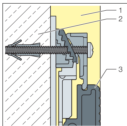
Fig. 19: Wall with 25 mm plaster layer
