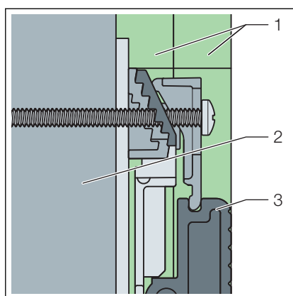
Fig. 21: Lightweight construction wall with two gypsum plaster boards, 12.5 mm each
