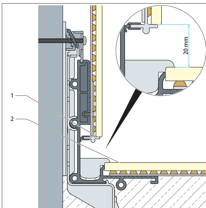
Fig. 23: Installed end strip, wall and floor tiles laid
