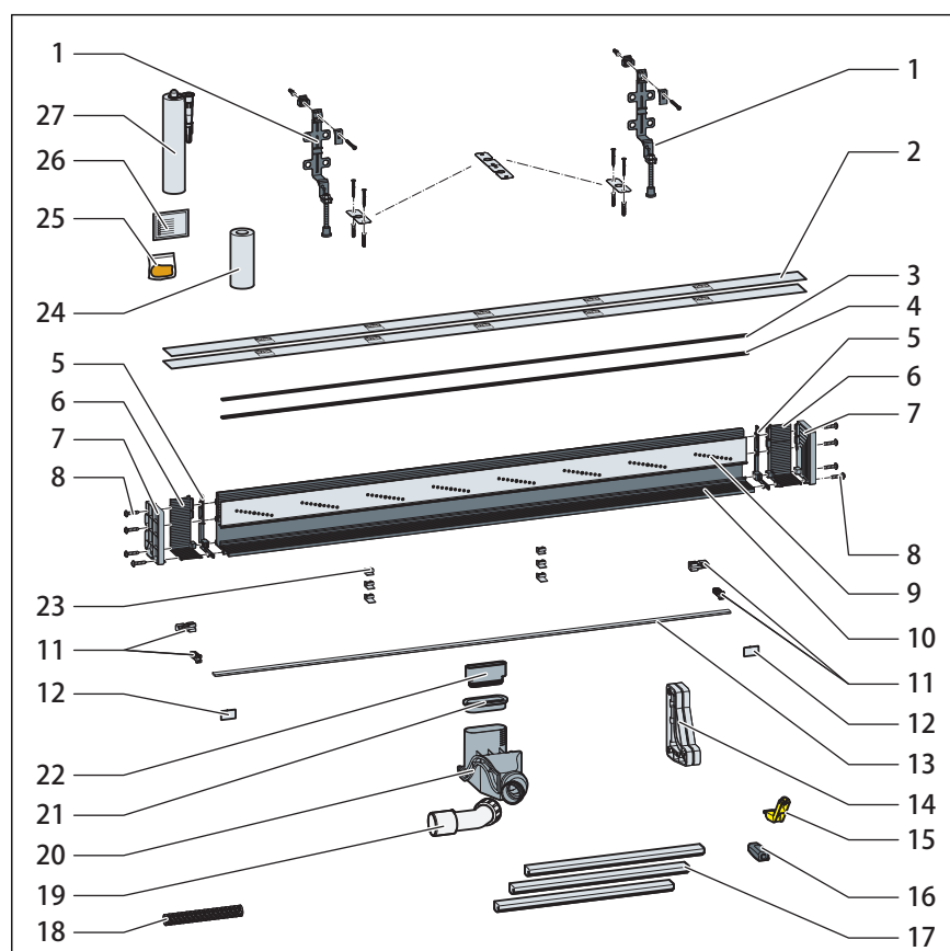
Fig. 13: Components and scope of delivery
