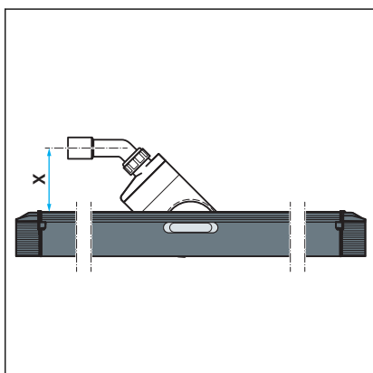
Fig. 11: Model 4965.85
