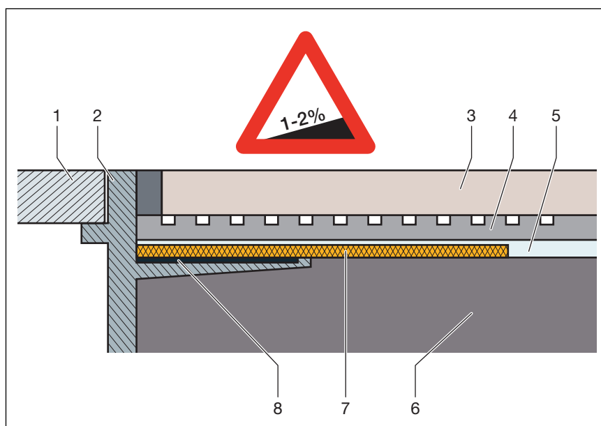
Fig. 15: Construction diagram of the bonded seal - min. screed incline 1–2 %
