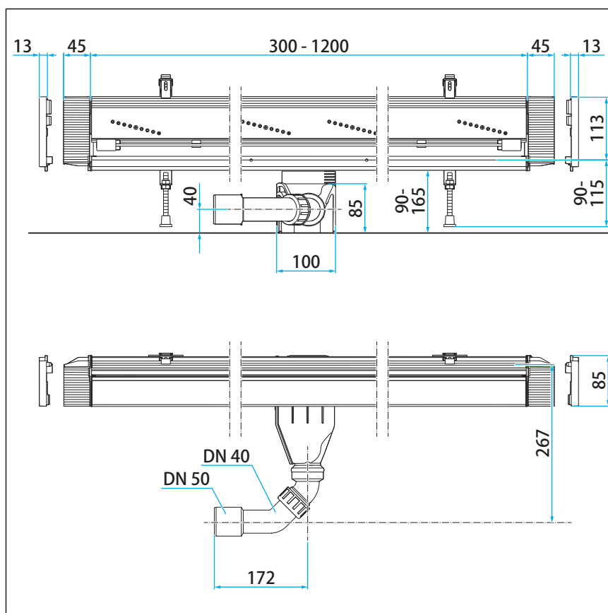
Fig. 18: Dimensions of base unit basic model
